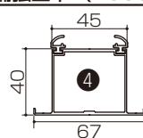
補強垂木F(1500)
