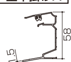
垂木掛けA
