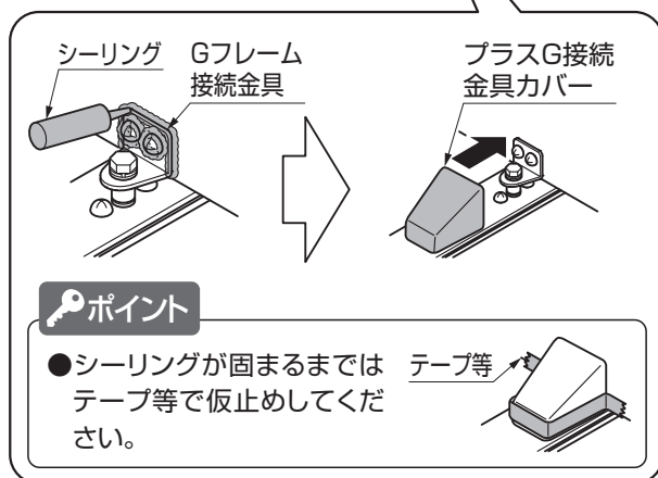
図7-2 A部 端部水下側
