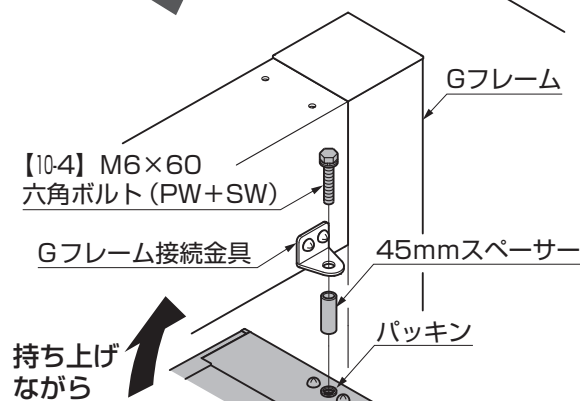
図7-2 A部 端部水下側
