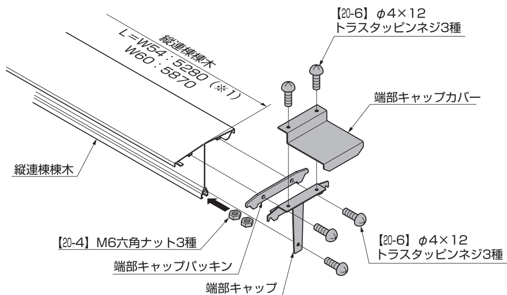
図2-7 縦連棟棟木の組立て
